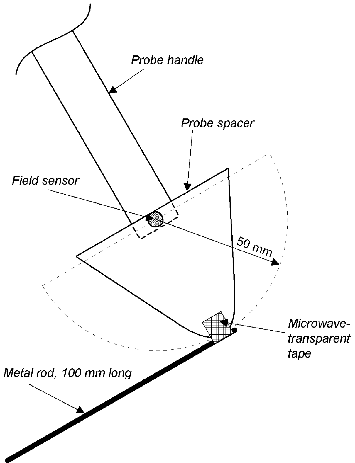
Arrangement for measuring microwave leakage from access openings
