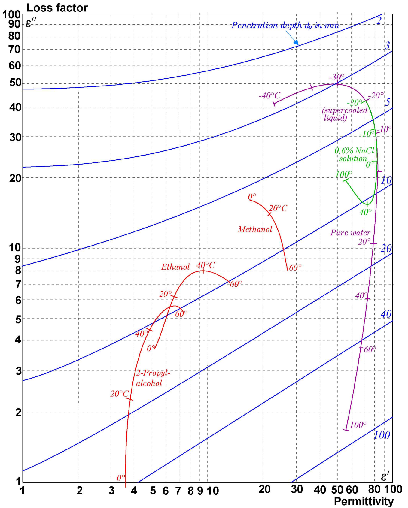
Complex permittivity diagram at 2450 MHz with d_p as parameter.
